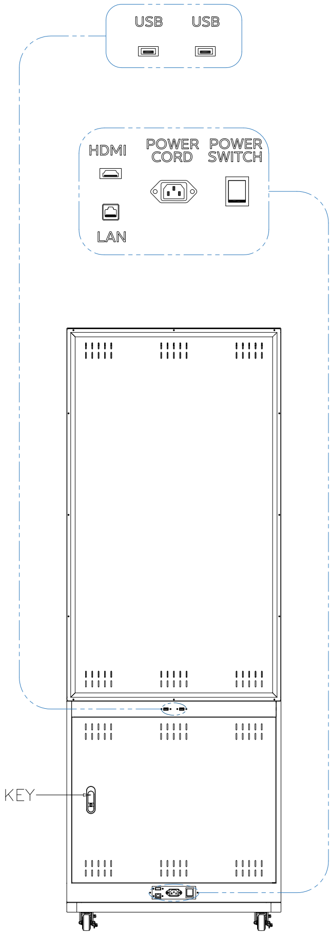
REAR VIEW
