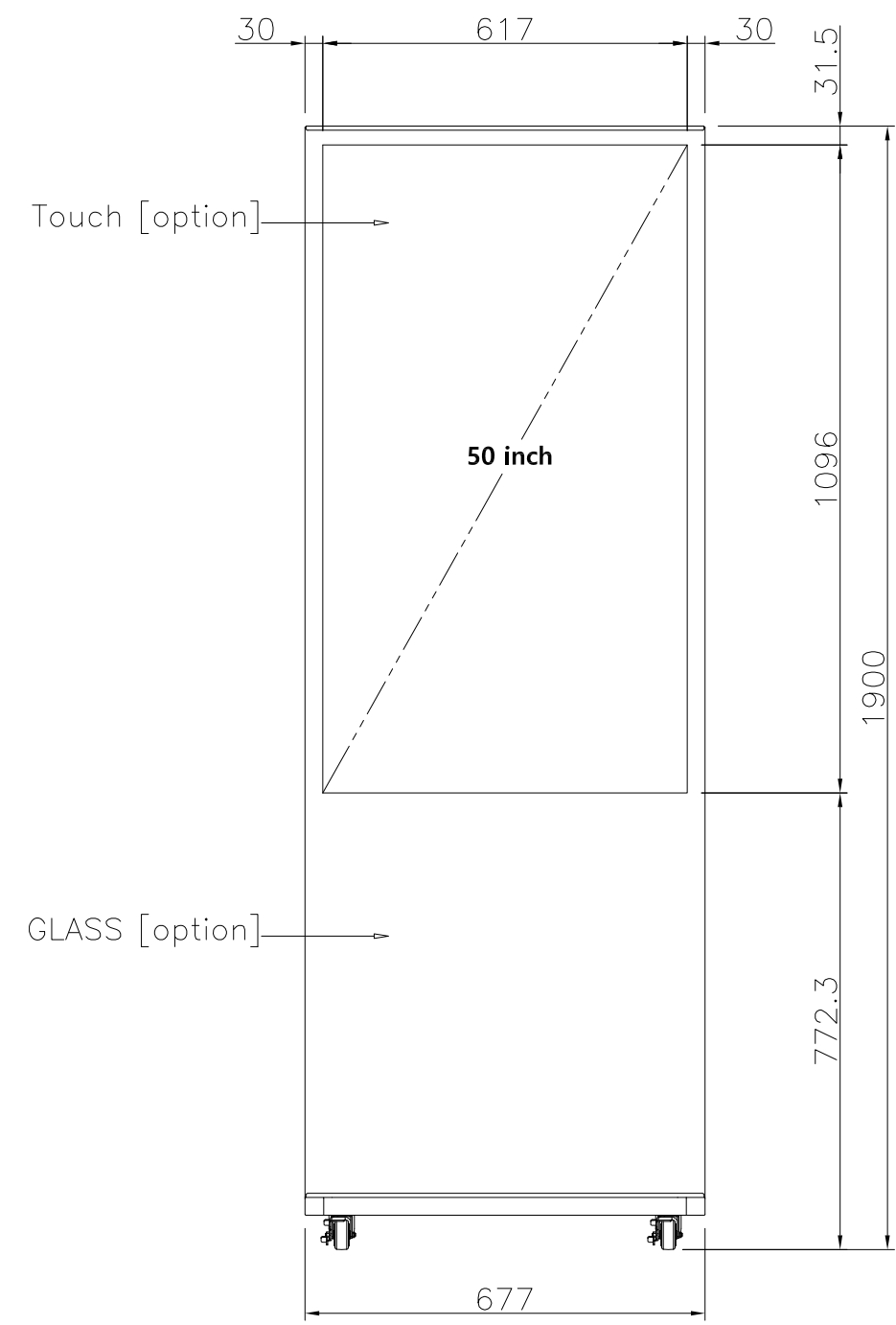
FRONT VIEW
